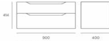
Double Drawer - Low SOLDWR.D.L
