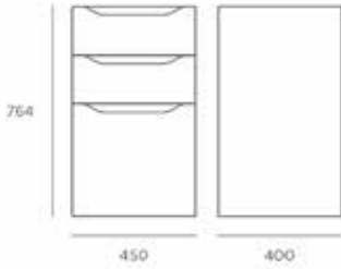
Single Drawer - High SOLDWR.S.H
