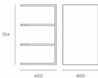
Single End Shelf - High - Left SOLESF.S.H.LFT
