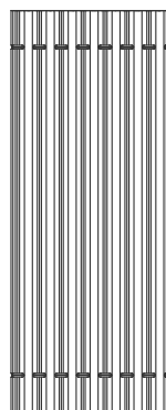
DWPN1650, high narrow
